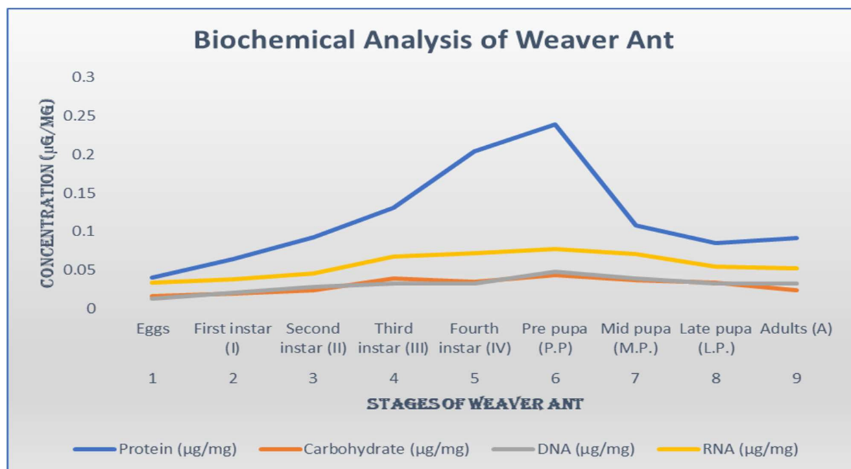
Figure 1: Total concentrations of protein, carbohydrate, RNA and DNA at various stages of Weaver
